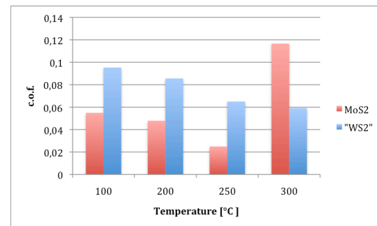
Figure 2. The average coefficient of friction values for ta-C coated LST surfaces with \text{MoS}_2 and \text{WS}_2 addition at different temperatures.
