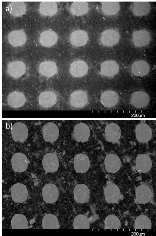
Figure 1. Burnished a) \text{MoS}_2 and b) \text{WS}_2 on ta-C coated LST steel surface.
