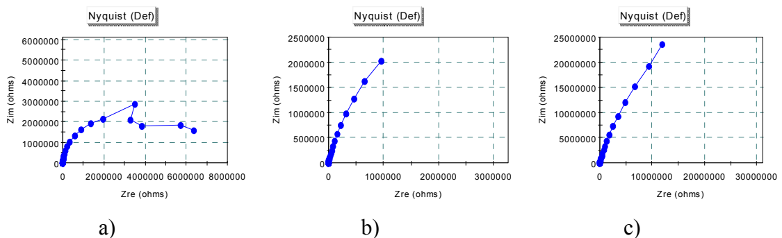
Fig. 3. Nyquist plots for a.)Zr, b.)Zr/ Al 2 O 3 , c.)Zr/ZrO 2 materials at SBF solution
