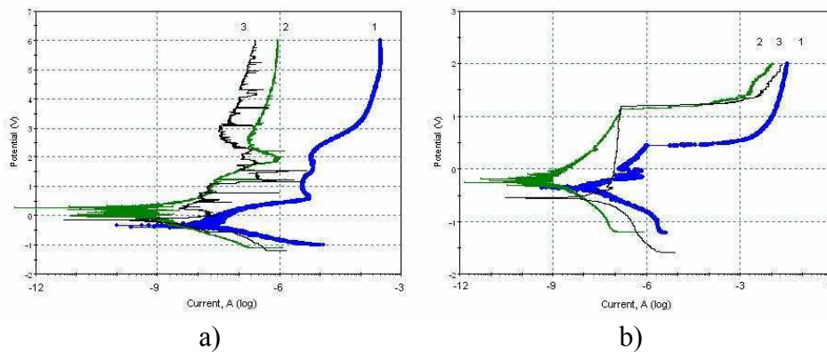
Fig. 2. The anodic polarization curves for a) 1-Ti, 2-Ti/ZrO 2 , 3-Ti/Al 2 O 3 , and b) 1-Zr, 2-Zr//ZrO 2 , 3-Zr/Al 2 O 3 coatings at SBF solution
