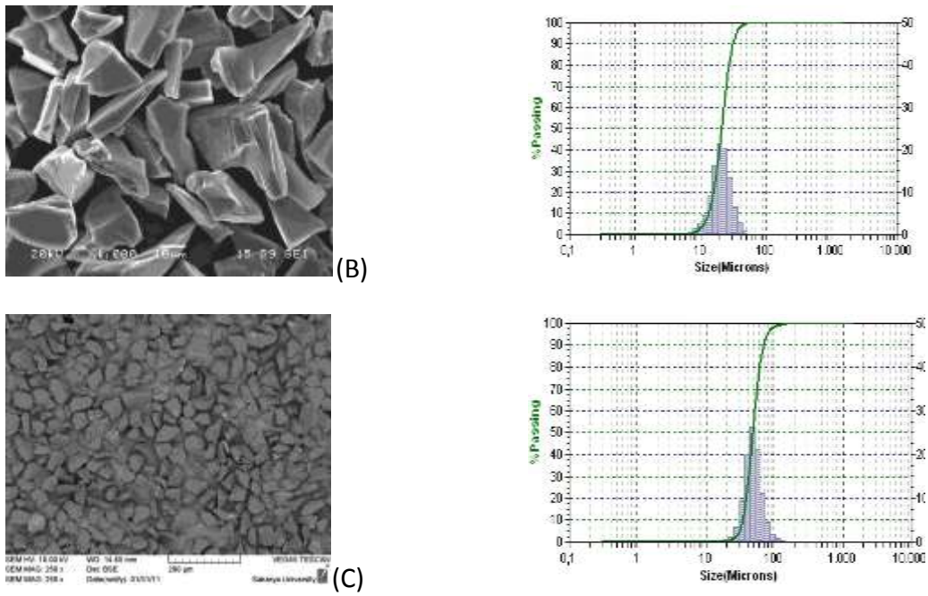
Figure 1 Powders SEM images and size distributions a) YSZ b) SiC c) B4C
