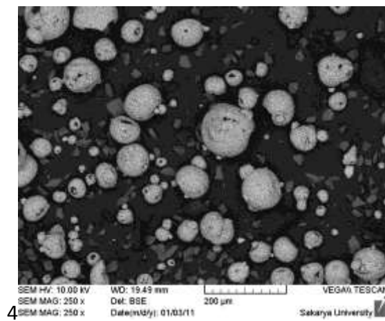
Figure 2 SEM image of %12,5 B4C and %12,5 SiC added YSZ
